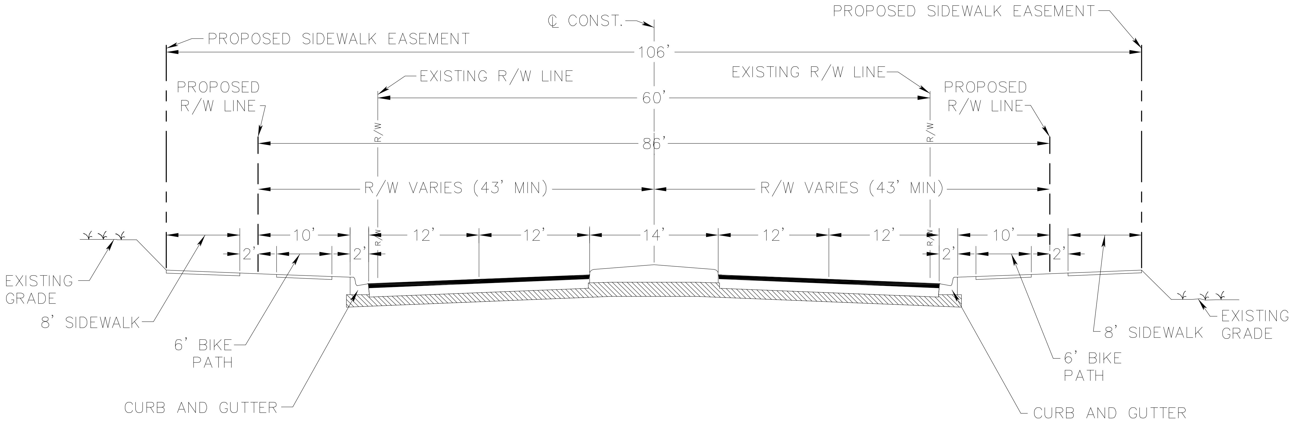
TYPICAL SECTION 60' RIGHT OF WAY
